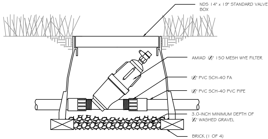
D 1 1/2" AMIAD 150 MESH WYE FILTER N.T.S. IN NDS STANDARD VALVE BOX 10.24.23 _wpl-nye-1.5
