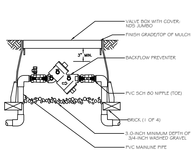
D WILKINS BACKFLOW PREVENTER N.T.S. 350FT SERIES 1/15/14 _wpl-d-bfp-950xlt
