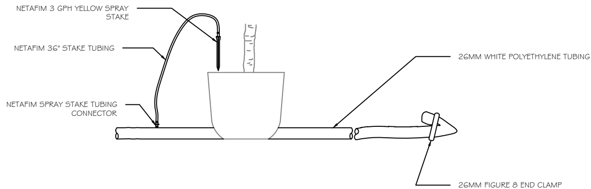
D NETAFIM 3 GPH SPRAY N.T.S. STAKES FOR POTS 10.24.23 _wpl-nye-1.5
