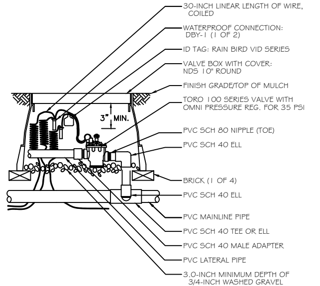
D TORO ELECTRIC VALVE 100 SERIES WITH N.T.S. OMNI PRESSURE REGULATOR (0-100 PSI) 12/9/10 wpl-d-v-tr-252
