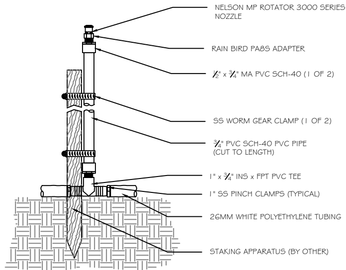
D NELSON 3000 SERIES MP ROTATOR N.T.S. MOUNTED ON RISER 10.24.23 _wpl-nye-1.5
